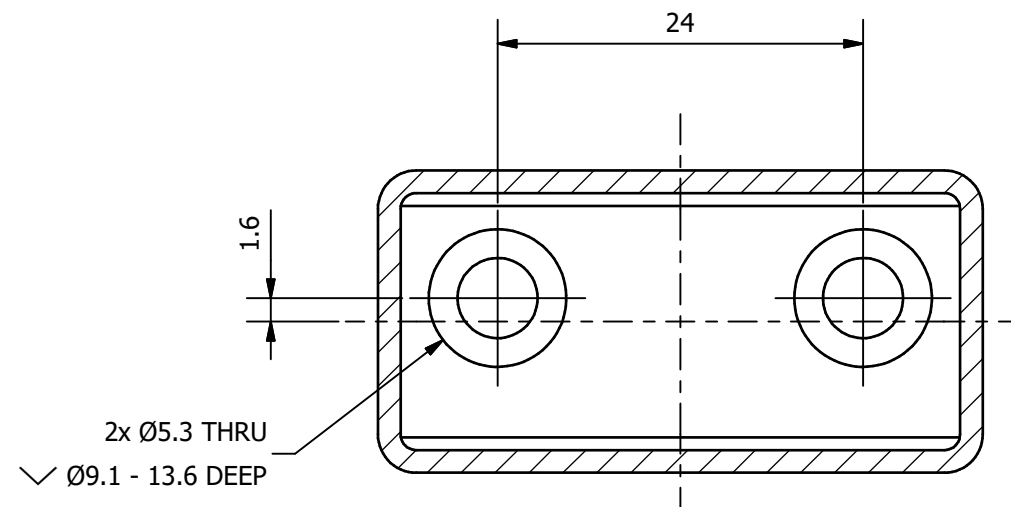
SECTION A-A MOUNTING DETAIL
